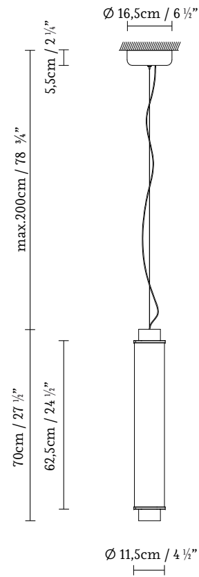
SLIM SKIN SV700
